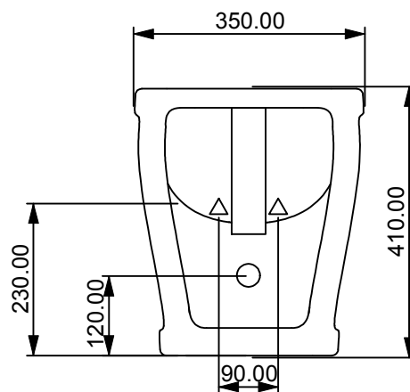
REAR
